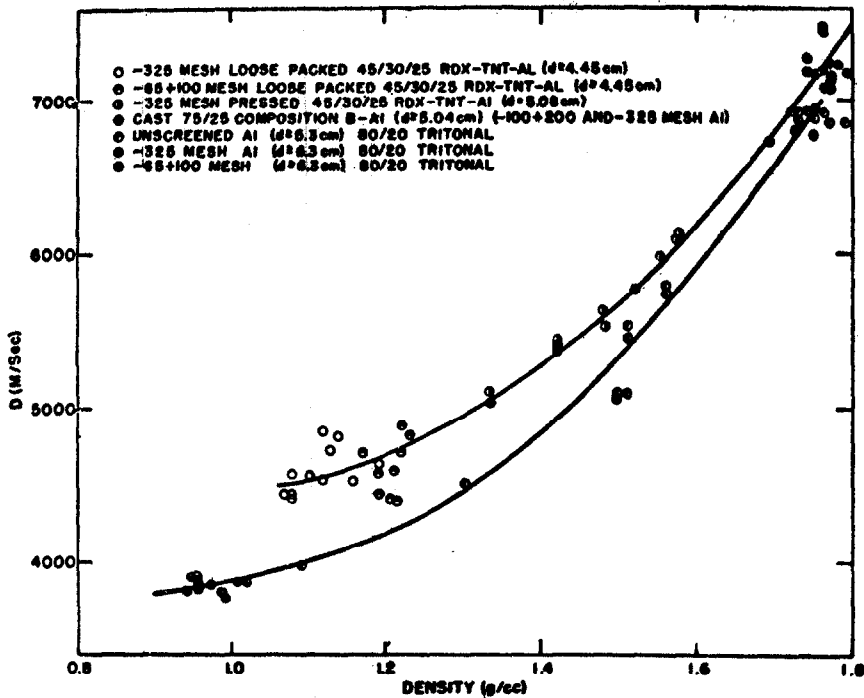
Figure 1 Velocity ( D ) versus density ( \rho_i ) curves for HBX and Tritonal
